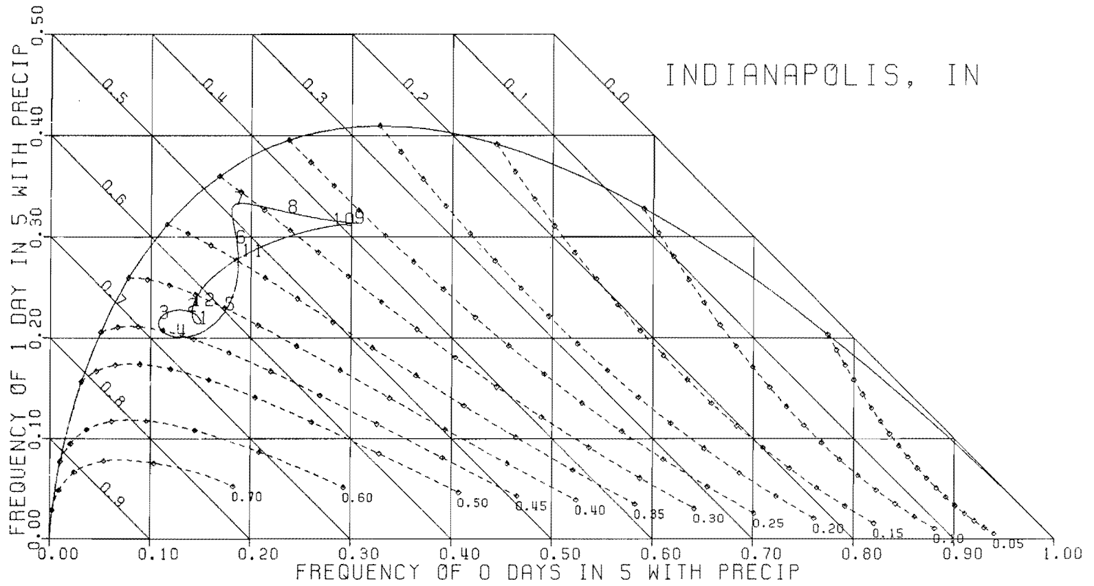
Figure 33. Same as Fig. 32, but for Indianapolis, IN. Note the weaker annual cycle and a wetter climate.
