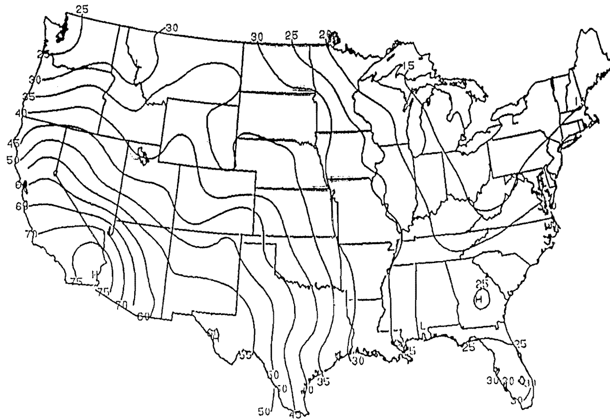
Figure 6. Mean annual relative frequency (%) of entirely dry 5-day periods over the conterminous United States.
