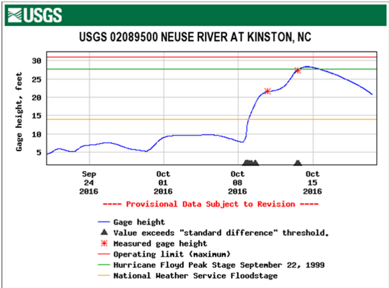
Figure 7: USGS graph of gage height or stage at stream gage 02089500 on the Neuse River at Kinston, NC, September 20 to October 20, 2016. Source: USGS
