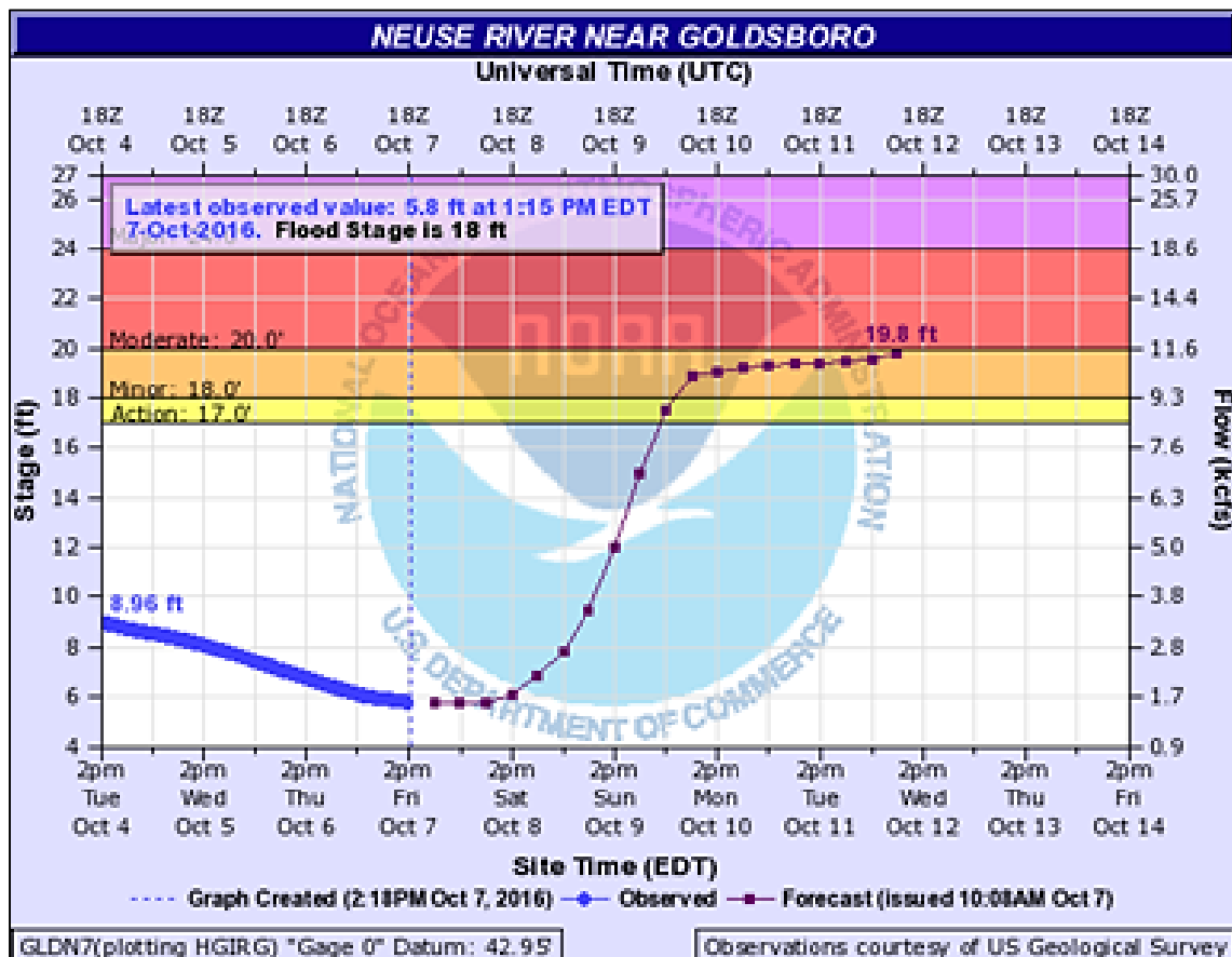
Figure 13: Advanced Hydrologic Prediction Service River Forecast, WFO Raleigh, NC, Friday, October 7, 2016 about 24 hours before heavy rainfall arrived. Source: NOAA
