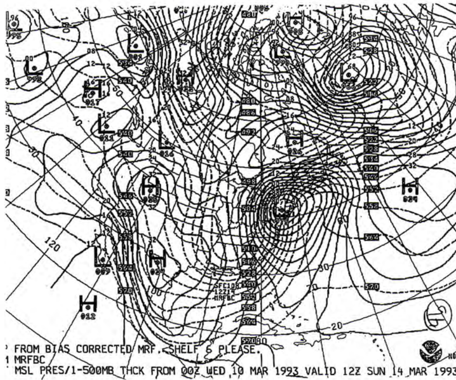
Surface Pressure
