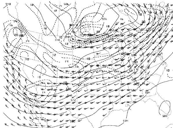
Figure 4. 4/21/96 12Z 500mb Heights/Vorticity (NGM)
