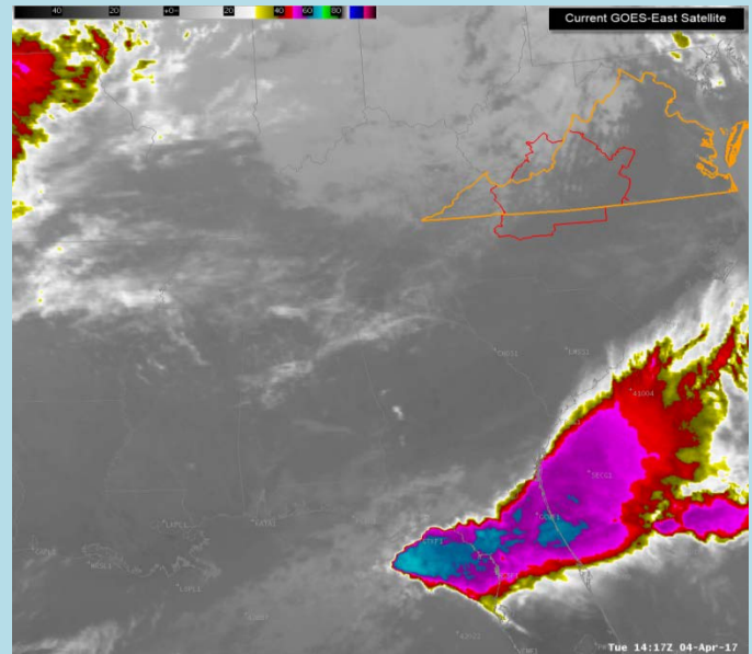
GOES-13 Infrared
