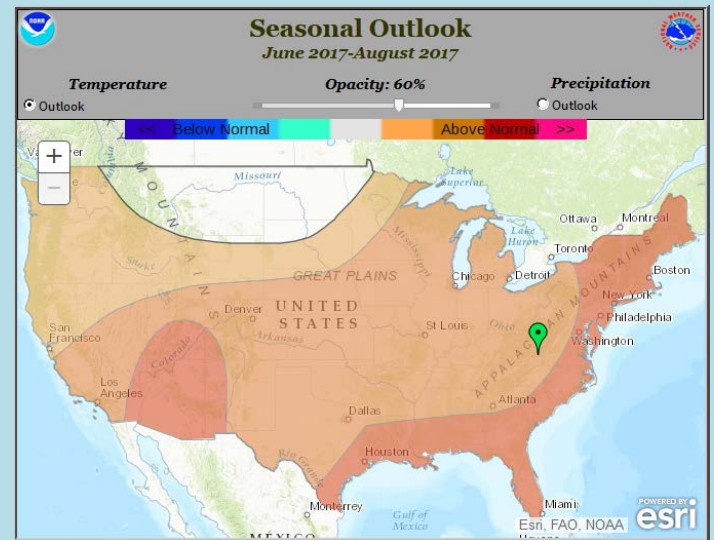
Summer Temperature Outlook (Jun-Aug)
