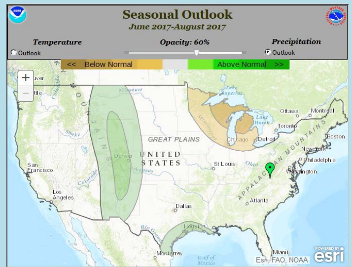
Summer Precipitation Outlook (June-Aug)
