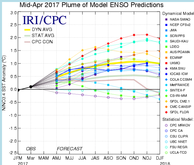
Model forecasts of ENSO through late 2017. Positive values indicate El Niño status while negative values indicate La Niña status
