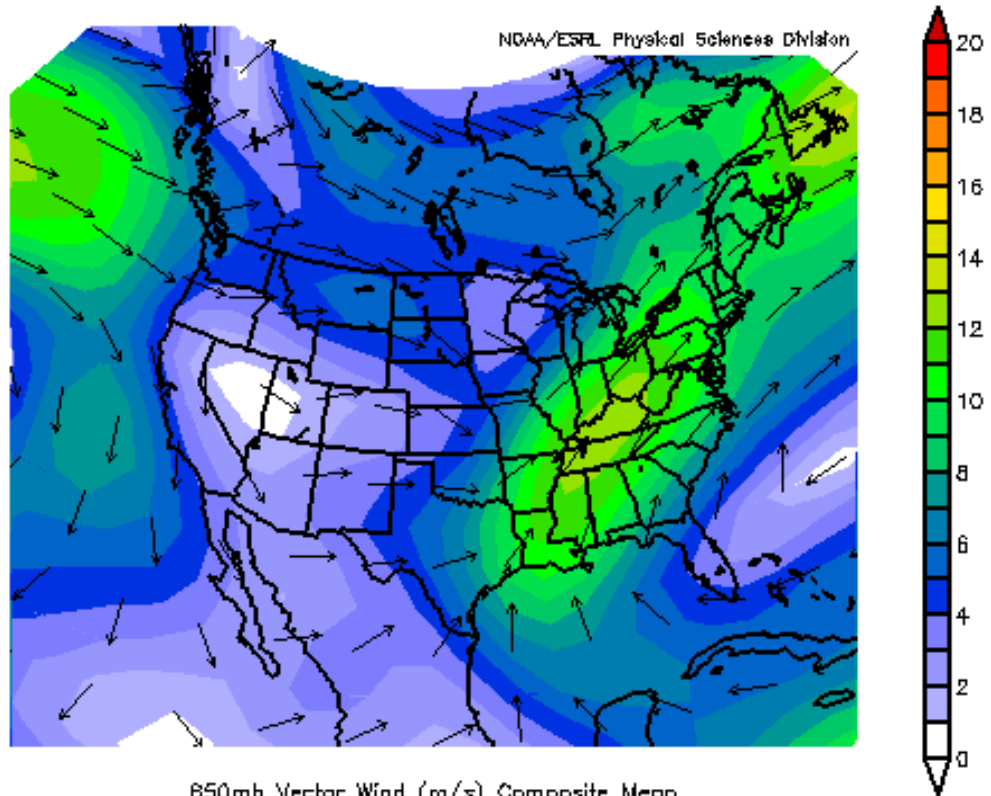
850mb Vector Wind (m/s) Composite Mean 9/9/74 12/29/74 11/7/96 11/27/01 2/17/75 10/26/64 11/7/69 2/15/05 2/18/75 1/20/62 2/8/86 2/ NCEP/NCAR Reanalysis
