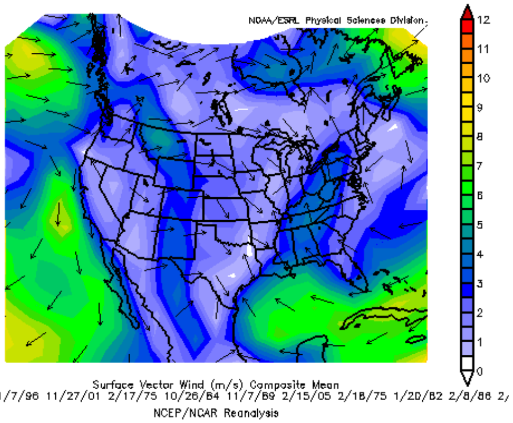
Figure 14. Surface wind speed ( \text{ms}^{-1} ) composite for all categories.
