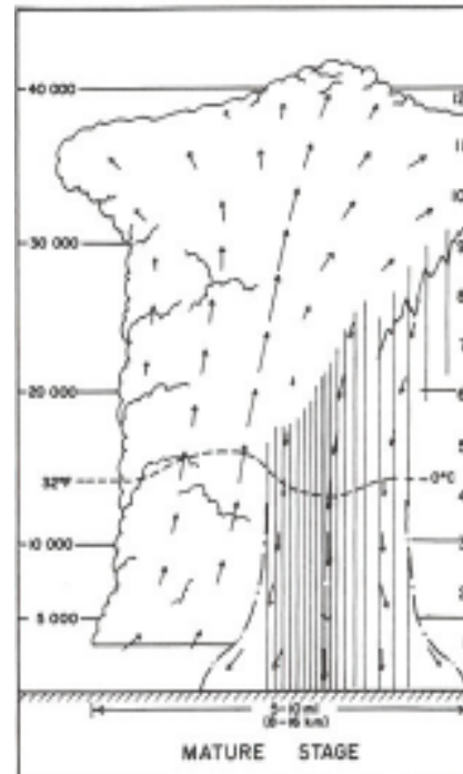
Figure 2: Mature stage of the thunderstorm. Updraft and downdraft are coexisting in the storm at this time.
