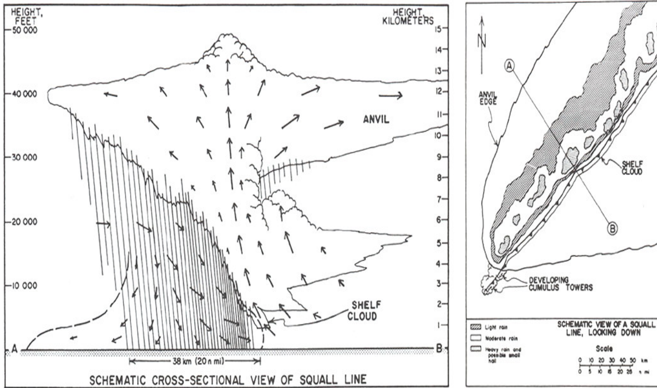
Figure 10: Schematic diagram of a squall line. Cloud outlines, radar intensities, and the area of greatest severe weather/tornado threat are shown.
