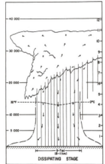
Figure 3: dissipating stage of the thunderstorm. Updraft has weakened and the storm is dominated by downdraft.
