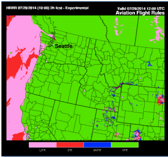
Figure 4 – HRRR forecast valid 12Z (5am PDT) Tuesday 29 July 2014. Areas shaded pink and red indicate IFR to LIFR ceilings.
