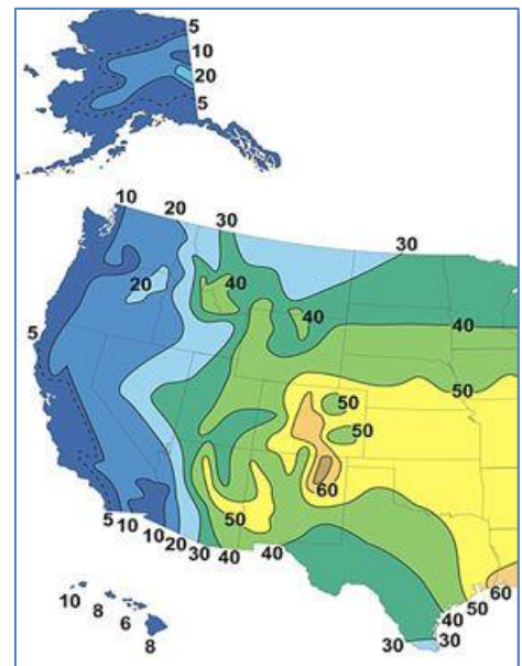
Figure 2 – Average number of thunderstorm days per year (from National Weather Service Southern Region).
