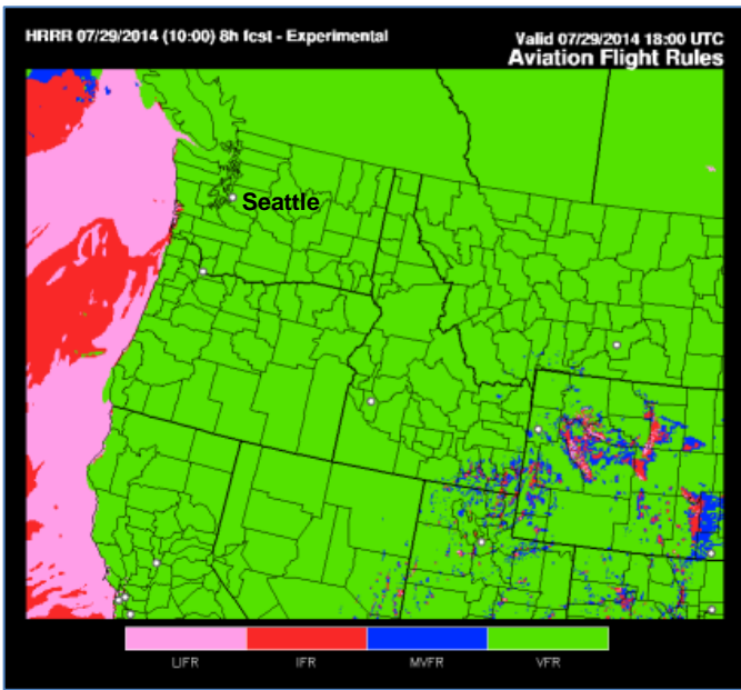
Figure 6 – HRRR forecast valid 18Z (11 am PDT) Tuesday 29 July 2014. Areas shaded pink and red indicate IFR to LIFR ceilings.
