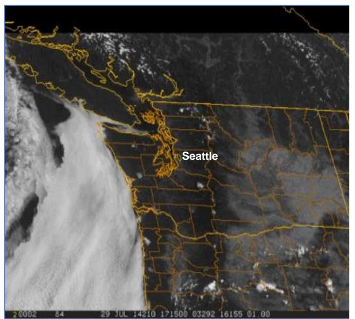
Figure 7 – Visible satellite image valid 1715Z 29 July 2014 showing low clouds in the Strait of Juan de Fuca and along the coast.
