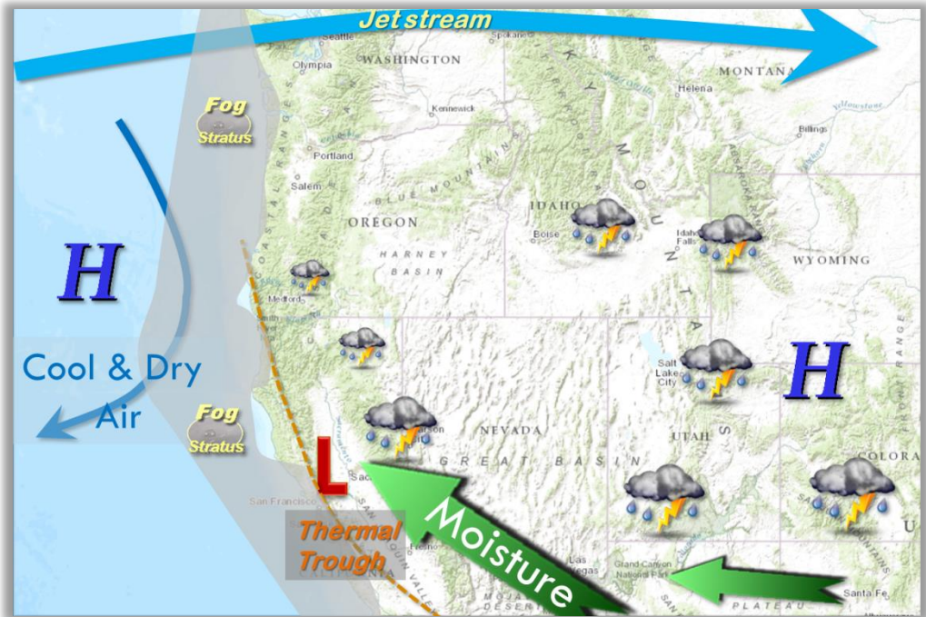
Figure 13 – Typical summertime pressure pattern and weather across the Western U.S.
