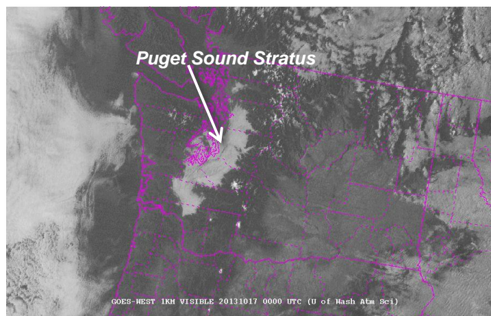
Figure 3 – Visible satellite image showing marine stratus over the interior lowlands of Western Washington
