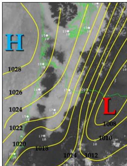
Figure 4 – Typical meteorological setup at the height of a marine stratus surge, showing the isobaric pattern of a thermal low pressure located in Columbia Basin.
